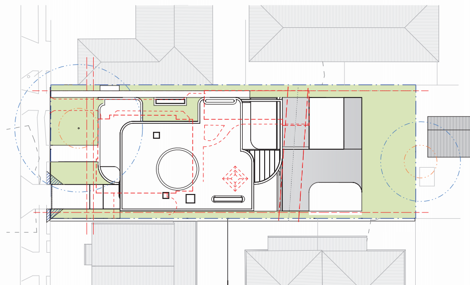
① SITE / DEMOLITION PLAN 1:200
